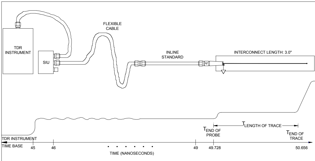
Figure 3 – Multiple: Find end of 3" Interconnect
