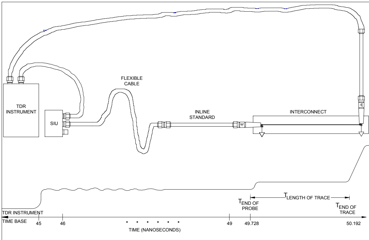
Figure 6 - TDT: Find end of Interconnect
