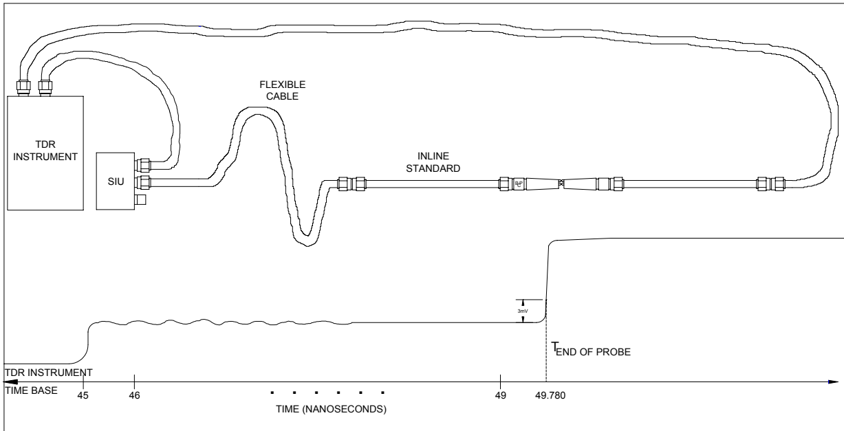
Figure 5 – TDT: Find End of #1 Probe
