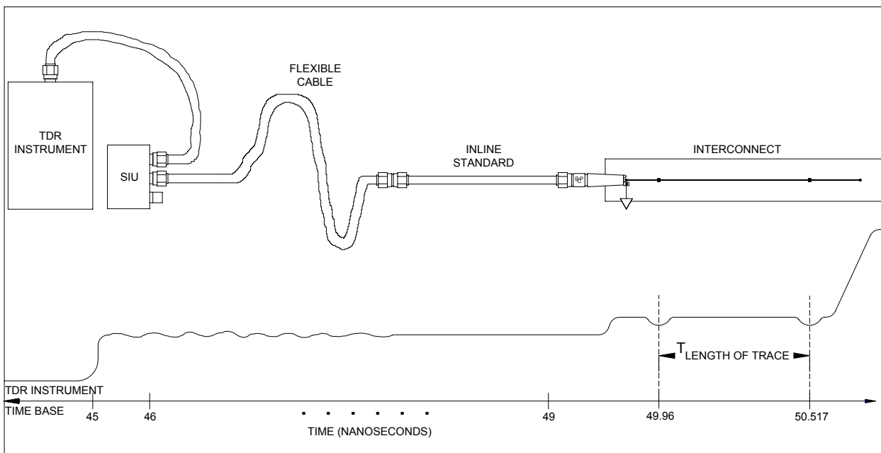
Figure 10 - Coupon: Measure start and end of interconnect segment
