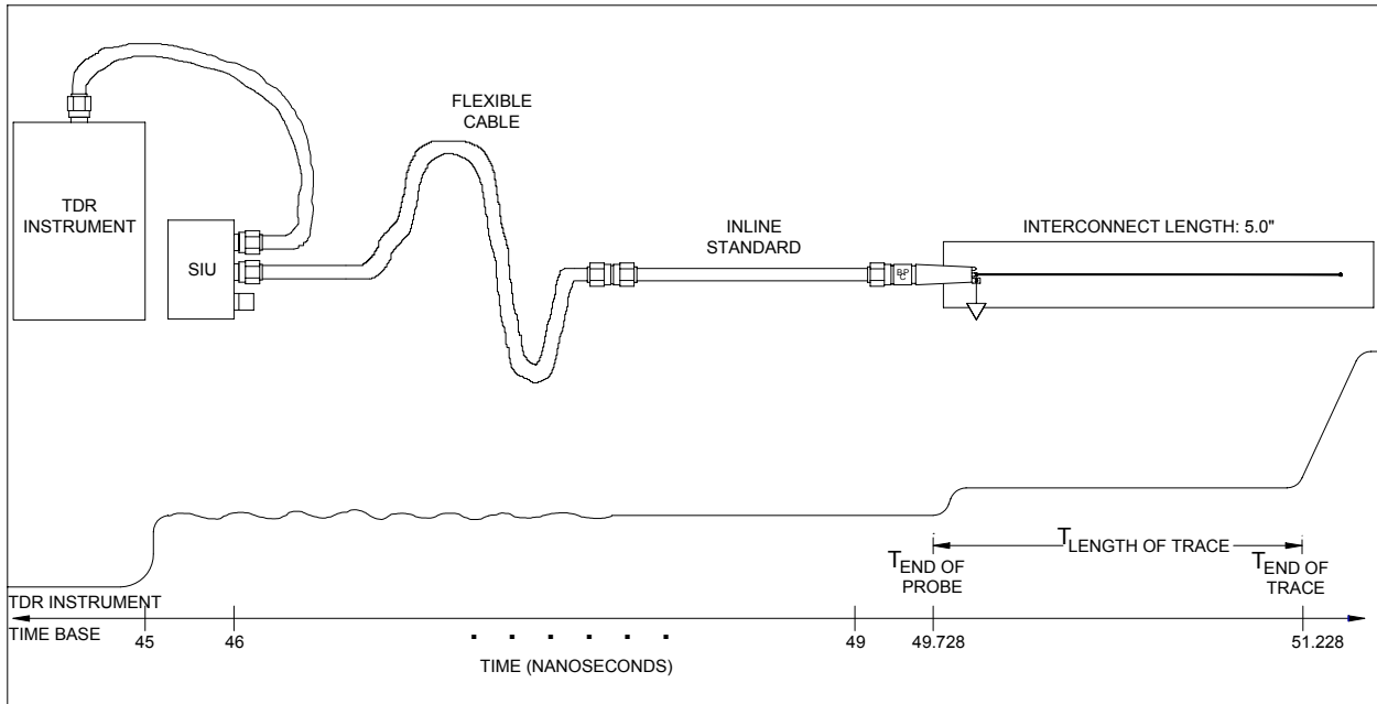
Figure 4 – Multiple: Find End of 5" Interconnect
