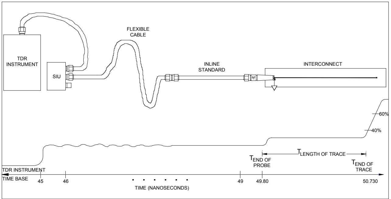
Figure 8 - TM-650: Find end of Interconnect
