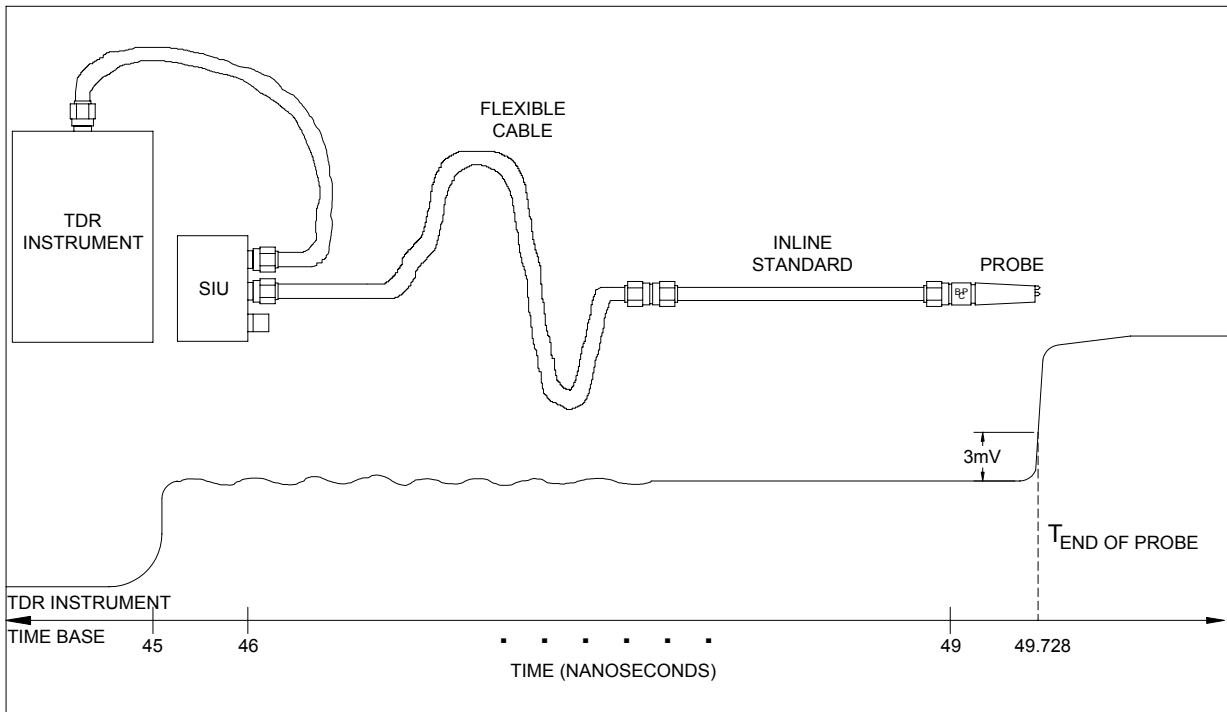
Figure 2 – Multiple: Find End of Probe
