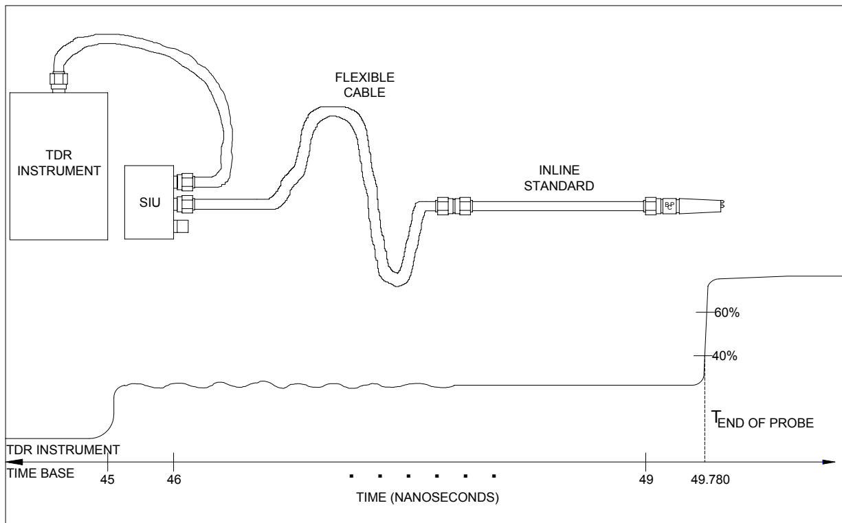
Figure 7 - TM-650: Find end of Probe
