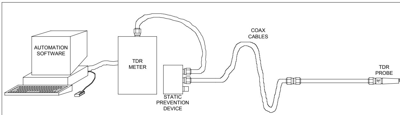
Figure 1 - TDR Equipment
