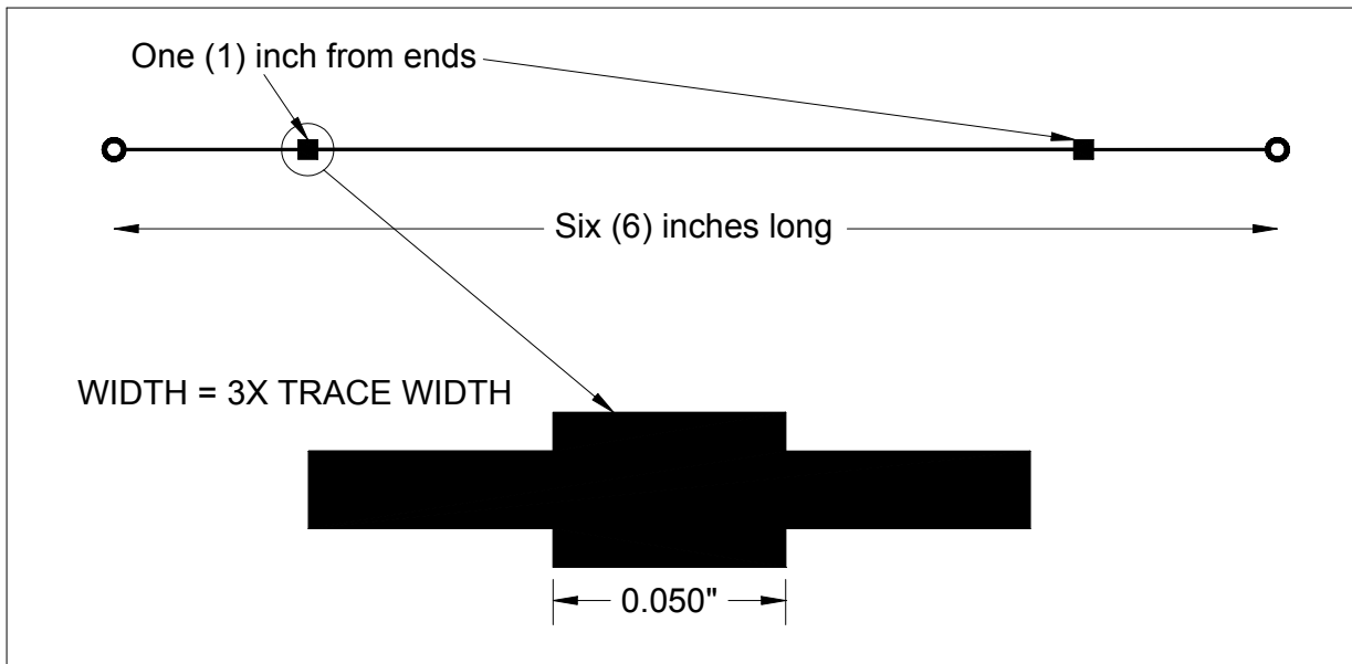
Figure 9 - Coupon Design
